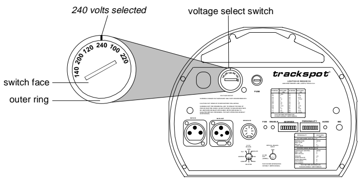
Figure 1-3. Trackspot rear panel
