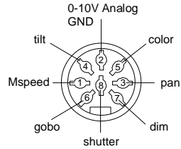
Figure 2-9. Analog In connector
